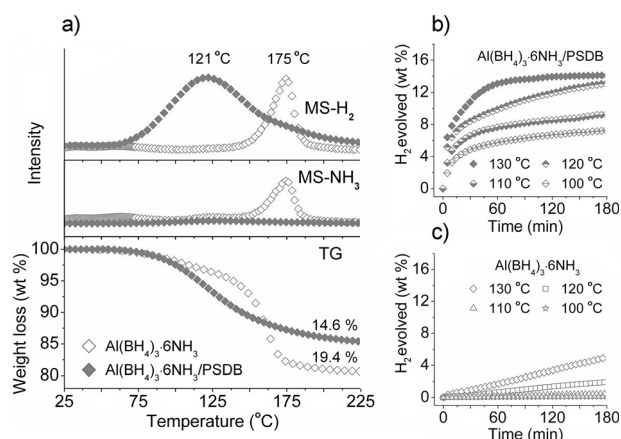
Figure 3. a) MS and TG profiles of \text{Al}(\text{BH}_4)_3\cdot 6\text{NH}_3/\text{PSDB} and bulk \text{Al}(\text{BH}_4)_3\cdot 6\text{NH}_3 with a heating rate of 5 °C min −1 . Isothermal TPD results of hydrogen released from \text{Al}(\text{BH}_4)_3\cdot 6\text{NH}_3/\text{PSDB} (b) and bulk \text{Al}(\text{BH}_4)_3\cdot 6\text{NH}_3 (c) at 100, 110, 120, and 130 °C (PSDB was not considered as a gravimetric component in the measurements).
